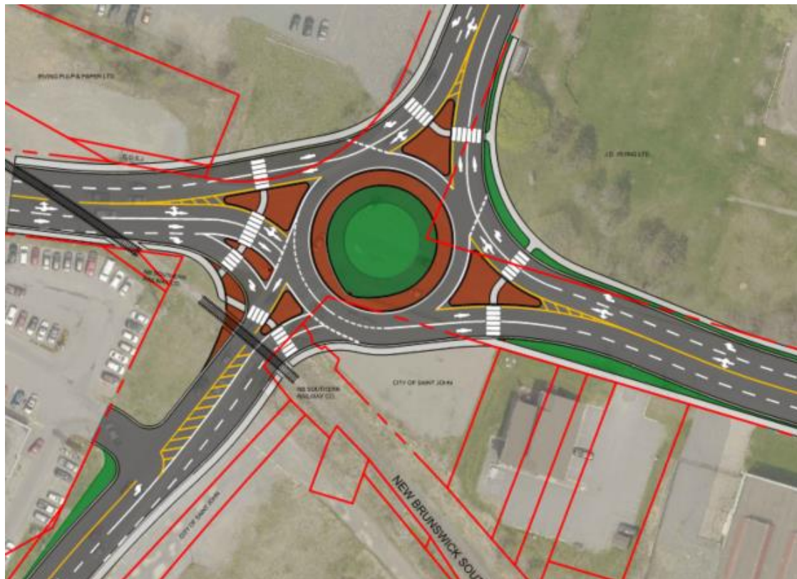
Exhibit 3.7: Simms Corner Roundabout Multi-Lane Roundabout Concept
